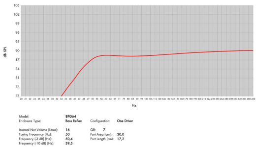
Frequency Response (1W/1m)
